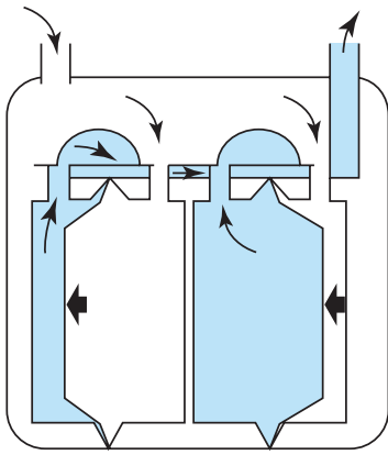
Working Principle
